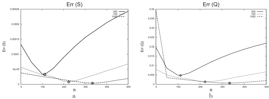
Figure 4. Error L^2 norms for (a) cross-section area ( S ) in \text{cm}^2 and (b) flow rate ( Q ) in \text{cm}^3 \cdot \text{s}^{-1} depending on the choice of R_{1D0D} (measured in \text{g} \cdot \text{cm}^{-4} \cdot \text{s}^{-1} ) in the 1D-0D-3D model for c_0 = 350, 700, 1050 \text{cm/s} . Circles mark results obtained with the choice of R_{1D0D} according to (13).
