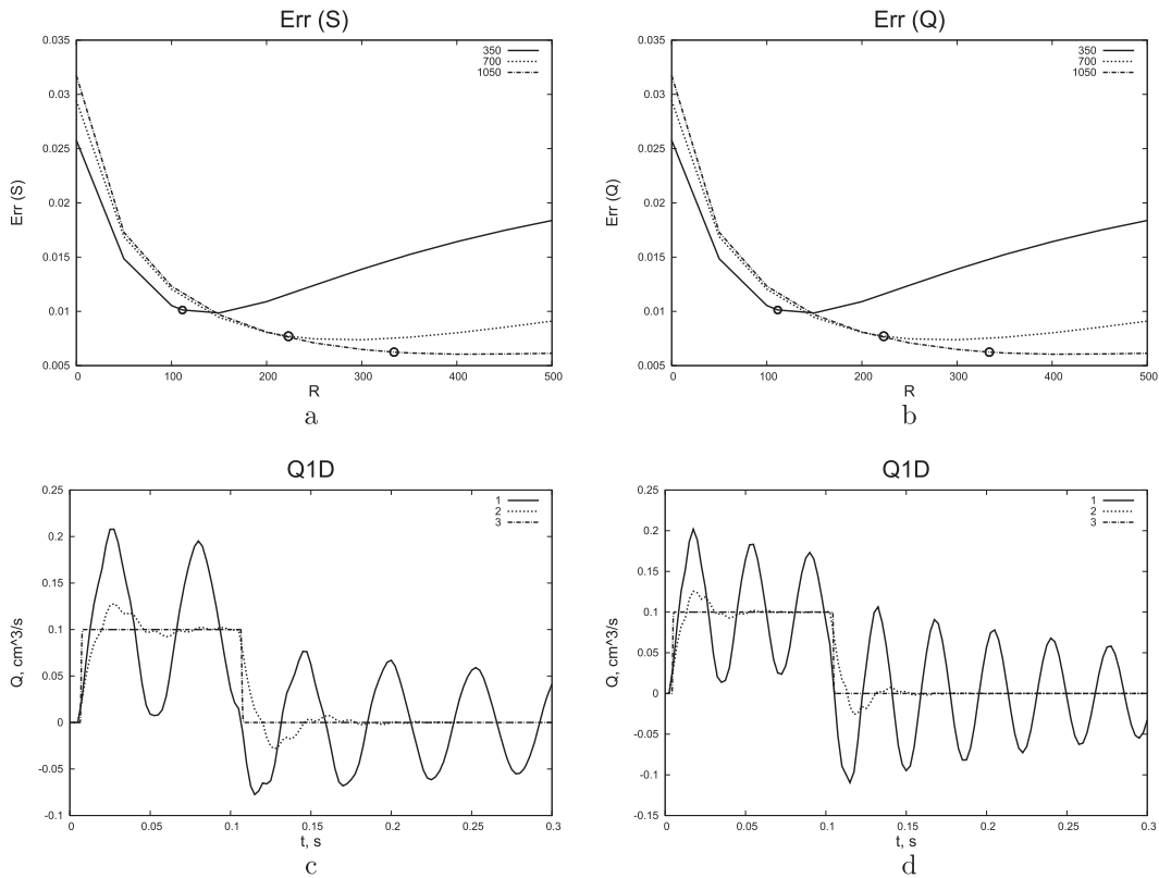
Figure 5. Step pulse wave experiment: Two upper figures show error L^2 norms for (a) cross-section area ( S ) in \text{cm}^2 and (b) flow rate ( Q ) in \text{cm}^3 \cdot \text{s}^{-1} depending on the choice of R_{1D0D} (measured in \text{g} \cdot \text{cm}^{-4} \cdot \text{s}^{-1} ) in the 1D-0D-3D model for c_0 = 350, 700, 1050 \text{cm/s} . Circles mark results obtained with the choice of R_{1D0D} according to (13). Figure 3(c)–(d) show time evolution of the flow rate at x = b computed with different models: (1) 1D-3D (hard coupling), (2) 1D-0D-3D (soft coupling), and (3) reference. Results are shown for several 1D elasticity parameters: Plot (c) is for c_0 = 700 \text{cm/s} , and plot (d) is for c_0 = 1050 \text{cm/s} .
