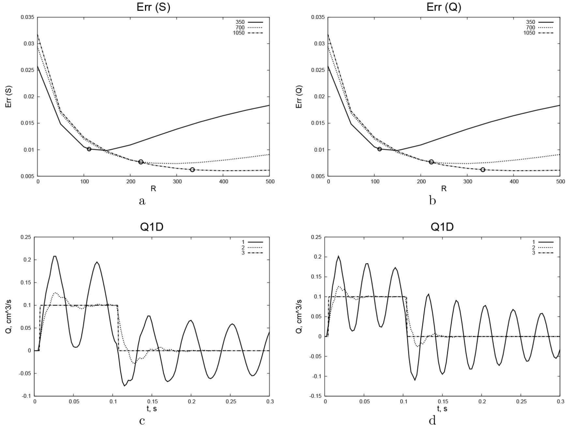
Figure 5: Step pulse wave experiment: Two upper figures show error L^2 norms for a) cross-section area (S) in cm 2 and b) flow rate (Q) in cm 3 · s -1 depending on the choice of R_{1D0D} (measured in g·cm -4 ·s -1 ) in the 1D-0D-3D model for c_0 = 350, 700, 1050 cm/s. Circles mark results obtained with the choice of R_{1D0D} according to (13). Figures c)–d) show time evolution of the flow rate at x = b computed with different models: 1) 1D-3D (hard coupling), 2) 1D-0D-3D (soft coupling) and 3) reference. Results are shown for several 1D elasticity parameters: plot c) is for c_0 = 700 cm/s, and plot d) is for c_0 = 1050 cm/s.
