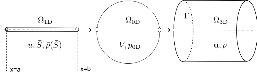
Figure 2: The schematic coupling of \Omega_{1D} , \Omega_{0D} and \Omega_{3D} domains.
