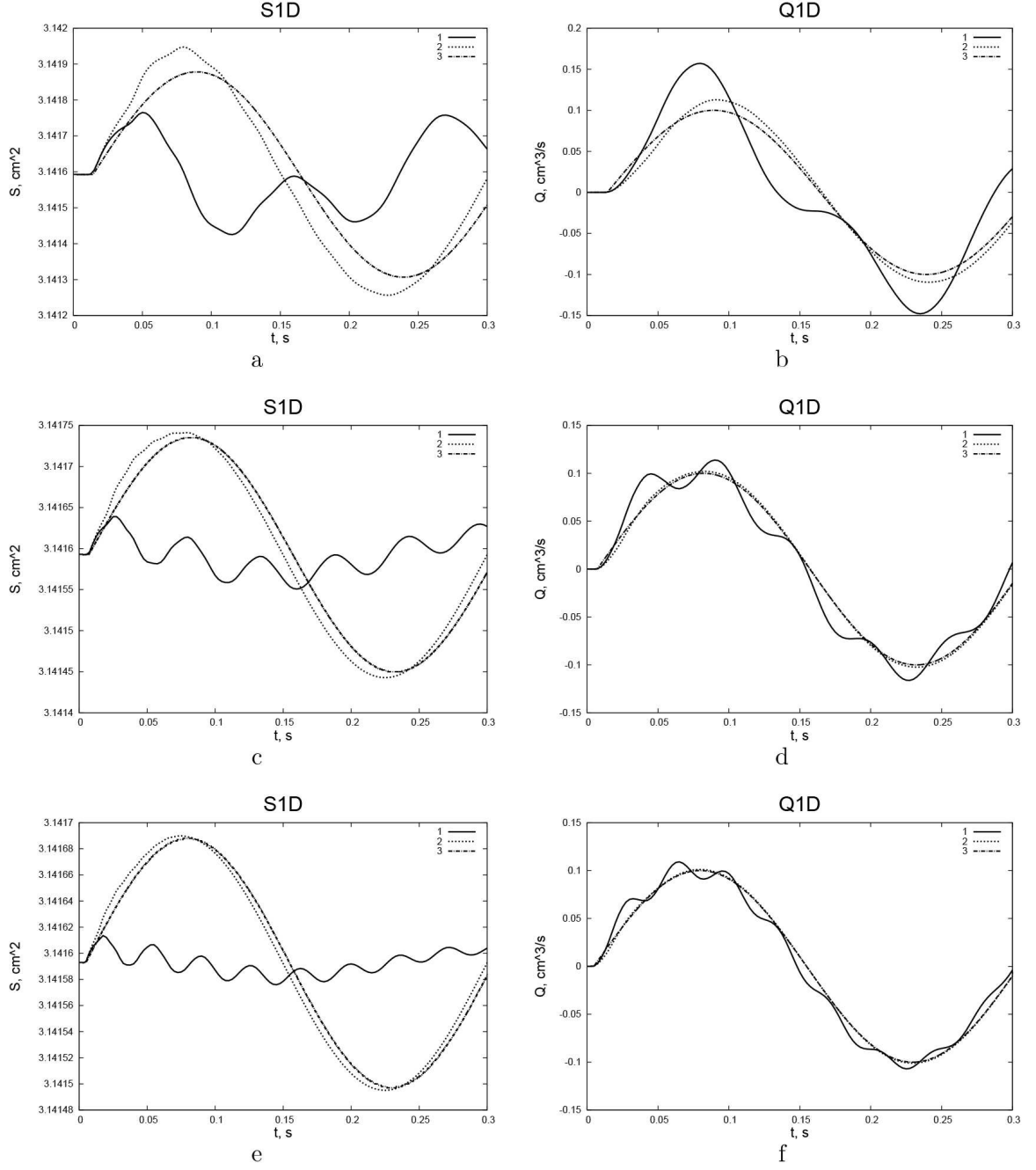
Figure 3: Time plots of the cross-section area and flow rate at x = b computed with different models: 1) 1D-3D (hard coupling), 2) 1D-0D-3D (soft coupling) and 3) reference. Results are shown for several 1D elasticity parameters: Plots a), b) are for c_0 = 350 cm/s, plots c), d) are for c_0 = 700 cm/s, and plots e), f) are for c_0 = 1050 cm/s.
