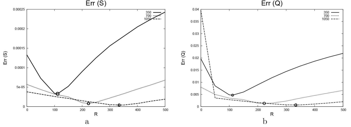
Figure 4: Error L^2 norms for a) cross-section area (S) in cm 2 and b) flow rate (Q) in cm 3 · s -1 depending on the choice of R_{1D0D} (measured in g·cm -4 ·s -1 ) in the 1D-0D-3D model for c_0 = 350, 700, 1050 cm/s. Circles mark results obtained with the choice of R_{1D0D} according to (13).
