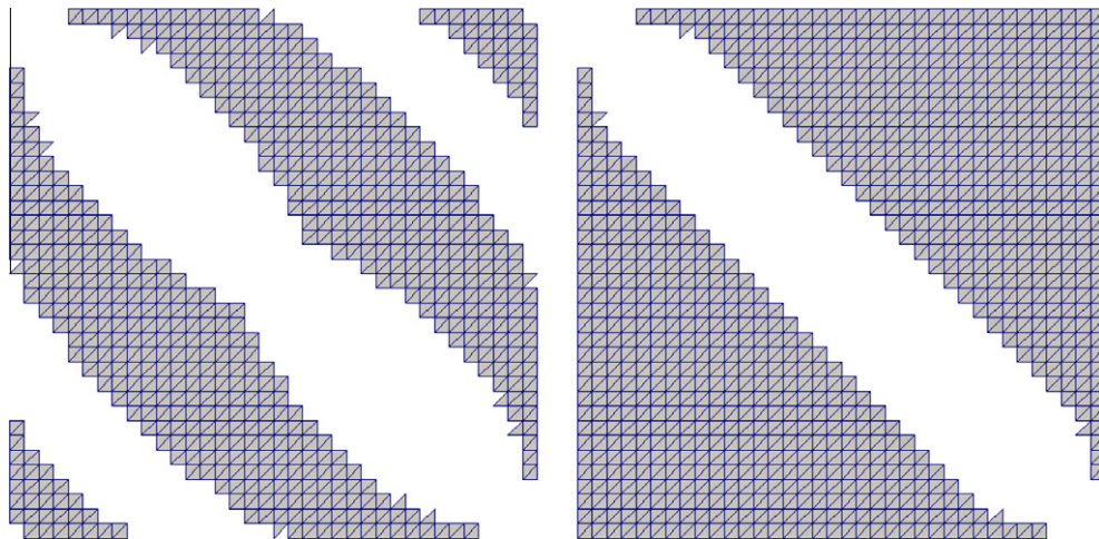
Fig. 11. Location of negative concentrations in the solutions to Problem 2: HMFEM (left) and monotonicity recovering (right).
