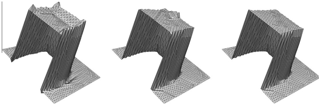
Fig. 5. SUPG solution to Problem 1 for \Delta t = 0.02 (left) and its postprocessed versions: with the non-negativity constraint C \geq 0 (center) and with the maximum principle constraint 0 \leq C \leq 1 (right).
