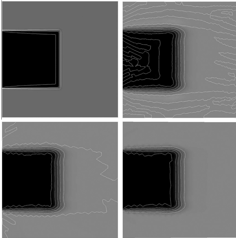
Fig. 3. Solutions to Problem 1: exact (top left), SUPG for \Delta t = 0.02 (top right), monotonicity recovering (bottom left), postprocessed for 0 \leq C \leq 1 (bottom right).
