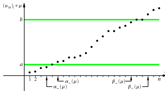
Fig. 2. The \mu -shift of u_M with the components (u_M)_i sorted in increasing order.
