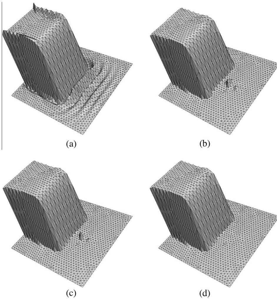
Fig. 8. (a) SUPG solution to Problem 1 for \Delta t = 0.005 ; and its postprocessed versions: (b) with one layer of neighbors; (c) with two layers of neighbors; (d) with two layers of neighbors and supplementary monotonicity constraints along the line y = 0 .
