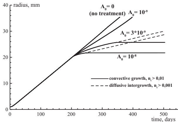
Figure 4. Dependence of the radius of the tumor on time for different levels A_0 of the preparation in the blood.
